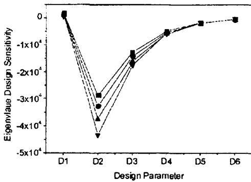
(a) First eigenvalue
