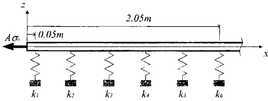
Fig. 6 A beam model for numerical simulation ; it is assumed that all supports are equally spaced and the beam section properties are not varying
