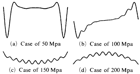
Fig. 9 First modes vs. different initial stresses ; when every spring constant is 100 kN/m, it can be seen that as the initial stress positively increases, irregular first mode shape becomes ordinary shape with fluctuation
